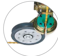
Wire can be placed enclosed in the machine
