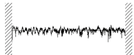
Surface superfinishing R_a = 0.051
